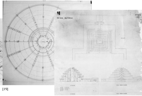
Section by Stanislas Jasinski
